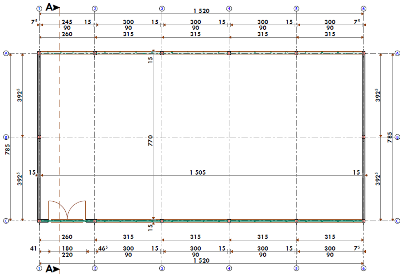
PLAN DE DISTRIBUTION - DISTRIBUTION PLAN
