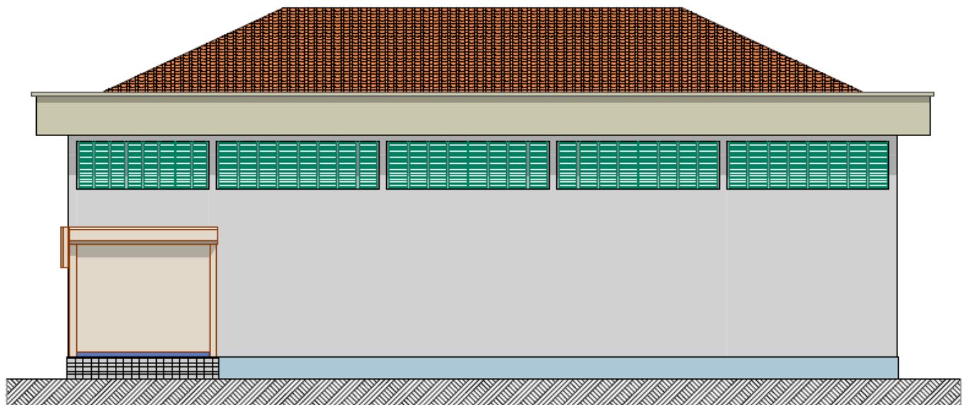
FACADE PRINCIPALE - FRONT ELEVATION
